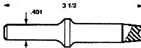
SOLID RIVET SETS
